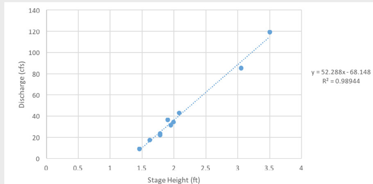
Figure 13: Stage-discharge curve from 12 observed measurements for Beaver Creek at the County Road G sampling location.
