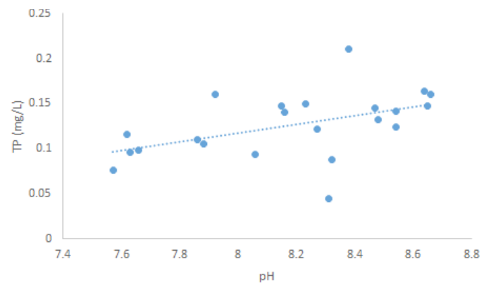
Figure 63: Relationship between TP and pH. The trendline equation is y = 0.0479x - 0.2658 and R^2 = 0.2287 .
