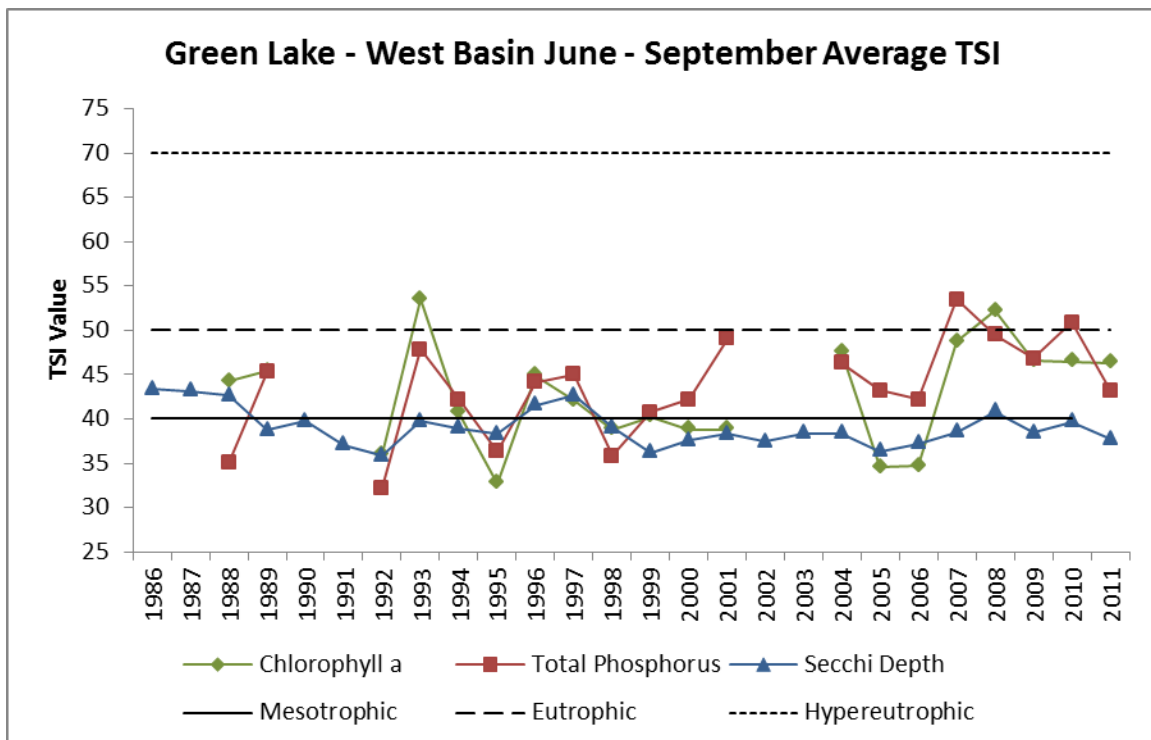
Figure 9 TSI (trophic state index) is a numerical value reflecting the nourishment level of a lake. The index values are on a 0 - 100 scale and reflect the levels of algae, phosphorous, and clarity in a lake. At Green Lake the TSI is generally in the 40 – 50 range, and considered mesotrophic, or mid-level of nourishment.
