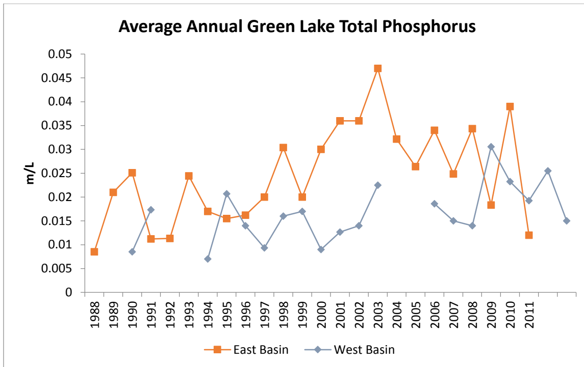
Figure 12 Green Lake total phosphorus (Sabai, A., SWIMS)
