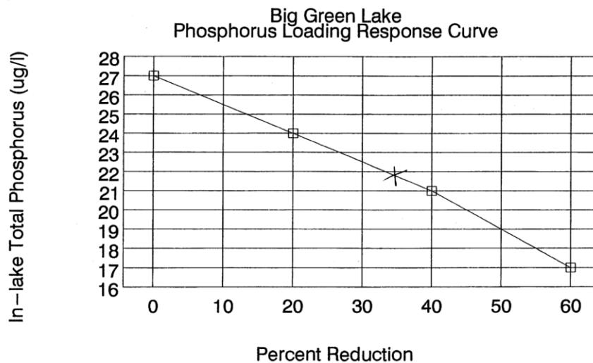
Figure 20 The regression curve above predicts Phosphorous response (in spring TP concentration) based on anticipated (target) reductions in total P loading to the lake (Panuska, J. 2001). The “X” approximates a 33% reduction in total P load to the lake. This target reduction, adopted by the GLSD in 2001, sets an objective for achieving a spring In-Lake Total P concentration of 22ug/L. Further evaluation monitoring is needed to determine how successful this previous effort has been. This plan includes objectives for improving evaluations of past and future efforts.
