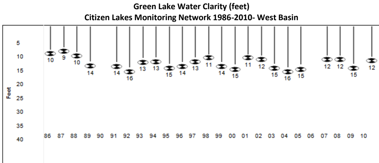
Figure 7 The above graph shows the annual average summer water clarity of Green Lake as measured by Secchi disc, over the past 25 years. The water clarity of the lake, despite the apparent annual variability, appears to be predictable, in the 10 to 16 foot range for average summer clarity (SWIMS data, WDNR). The average value does not indicate the maximum or minimum readings which could exceed 16 feet or be less than 10 feet on a particular day.
