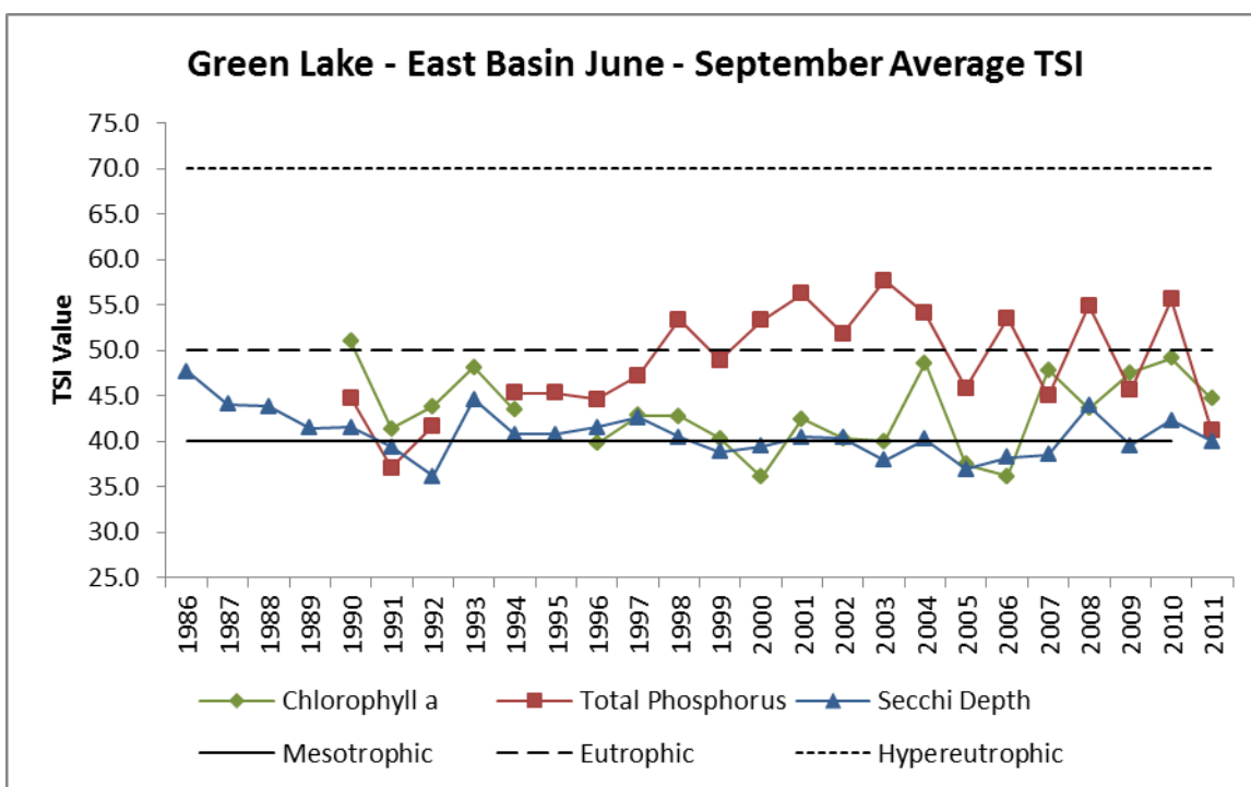
Figure 8 TSI (trophic state index) is a numerical value reflecting the nourishment level of a lake. The index values are on a 0 - 100 scale and reflect the levels of algae, phosphorous, and clarity in a lake. At Green Lake the TSI is generally in the 40 – 50 range, and considered mesotrophic, or mid-level of nourishment.
