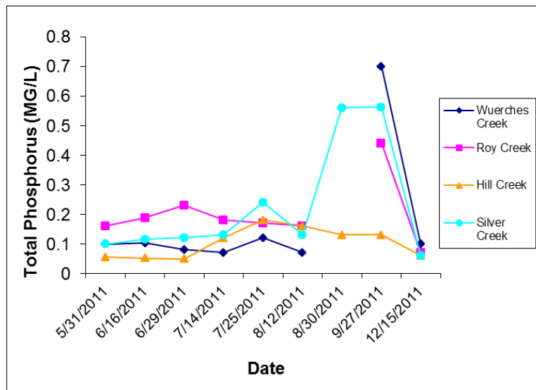
Figure 14 Total P concentrations of streams entering Green Lake. Most of the sampling was conducted under base flow conditions. The high concentrations from the 9/27 event reflect runoff from rains.
