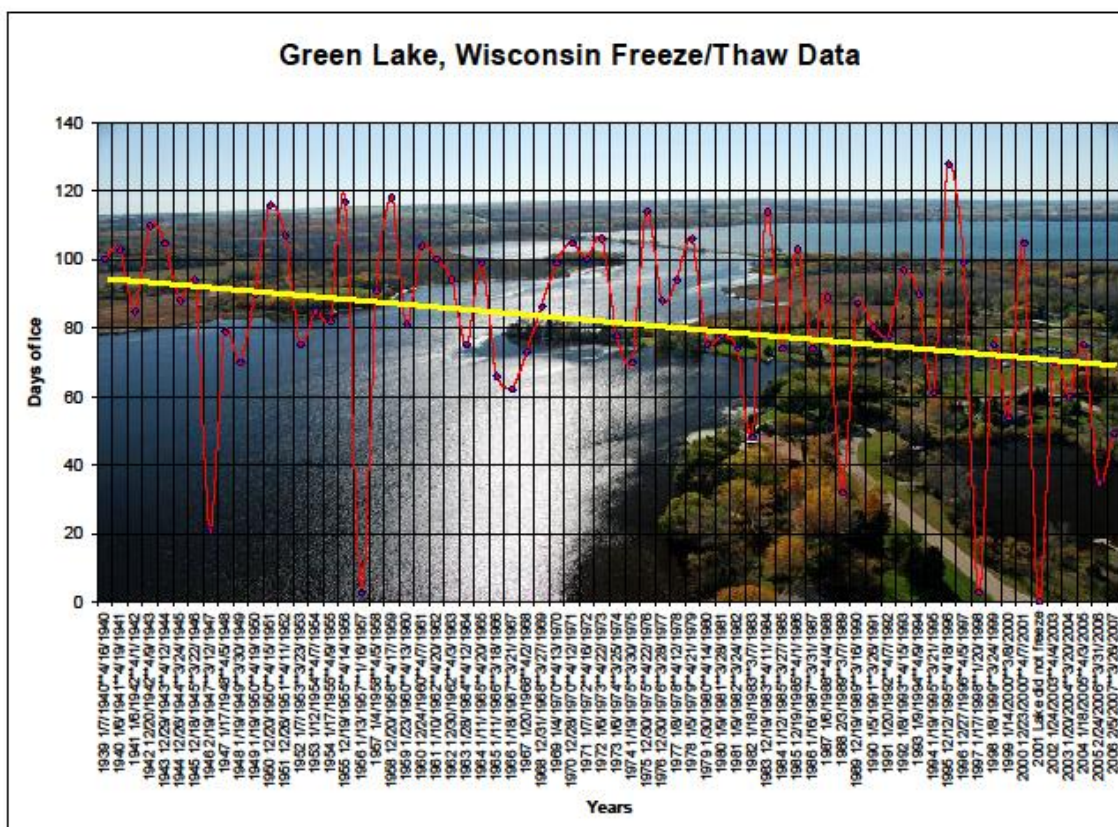
Figure 23 The duration of ice cover on Green Lake is decreasing as seen in the trend line above. The graph covers a period from 1940 through 2007 or 66 years of record. Similar trends are occurring on Lake Mendota and other Wisconsin lakes (Eddy, T).
